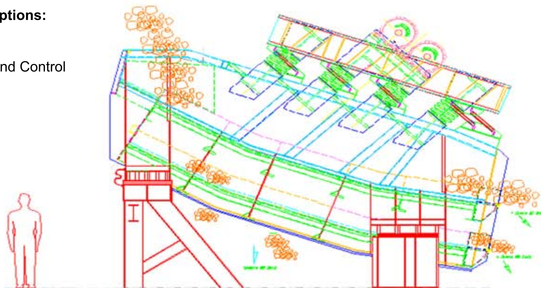
Banana Screen - Typical Arrangement
